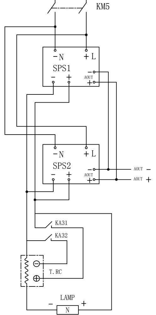
Xenon Lamps Circuit
