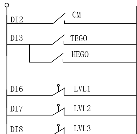
Protection Circuit
