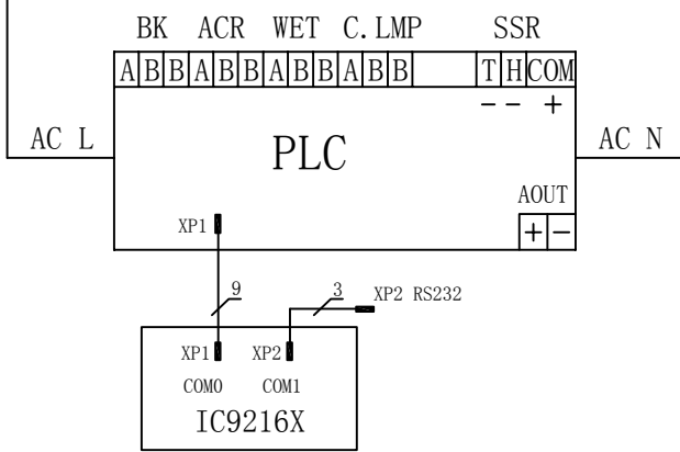
Total Circuit
