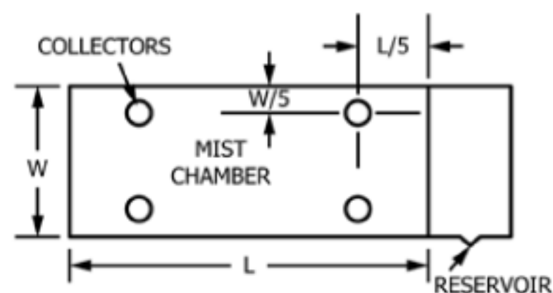
FIG. 1 Arrangement of Fog Collectors
